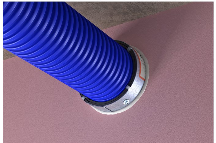
QRS Semi-rigid Fire Sleeve installed in plasterboard partition
